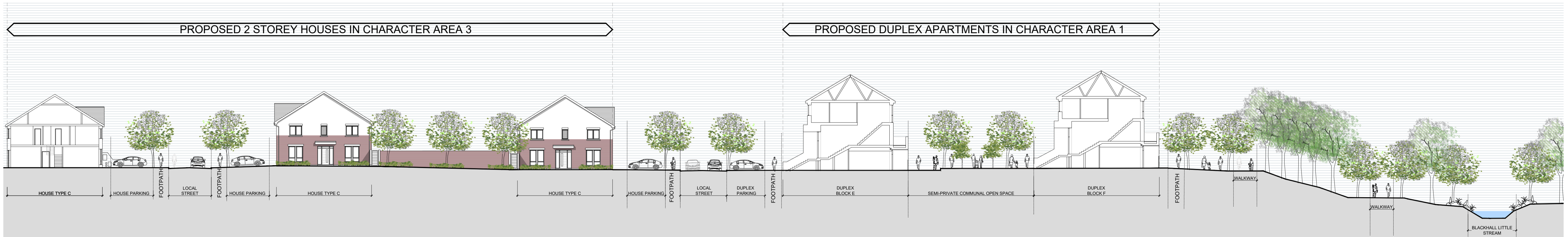
Site Section FF
