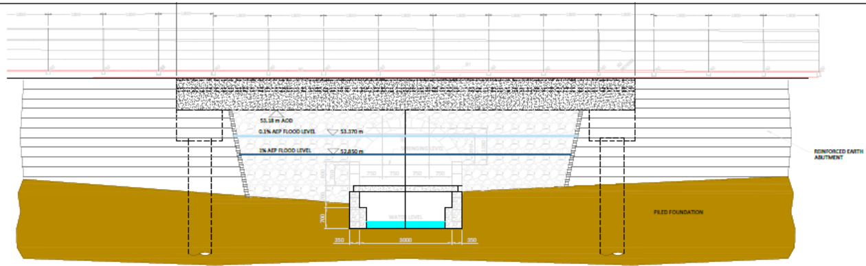
PROPOSED ELEVATION
