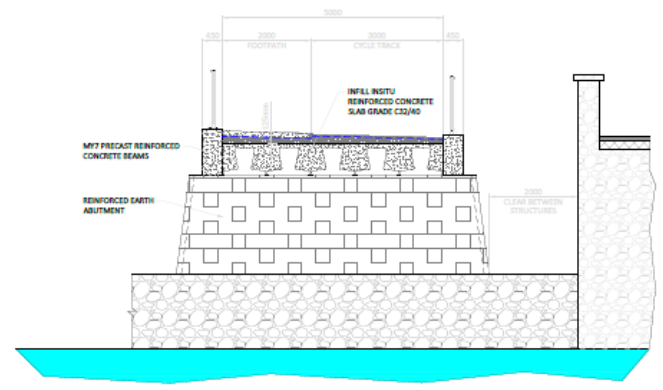
ABUTMENT ELEVATION SCALE 1:50
