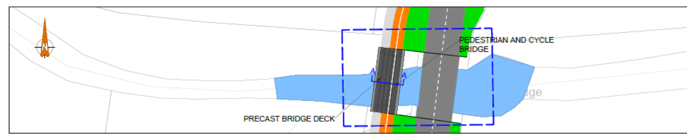
RYE RIVER PEDESTRIAN AND CYCLE BRIDGE SCALE 1:200
