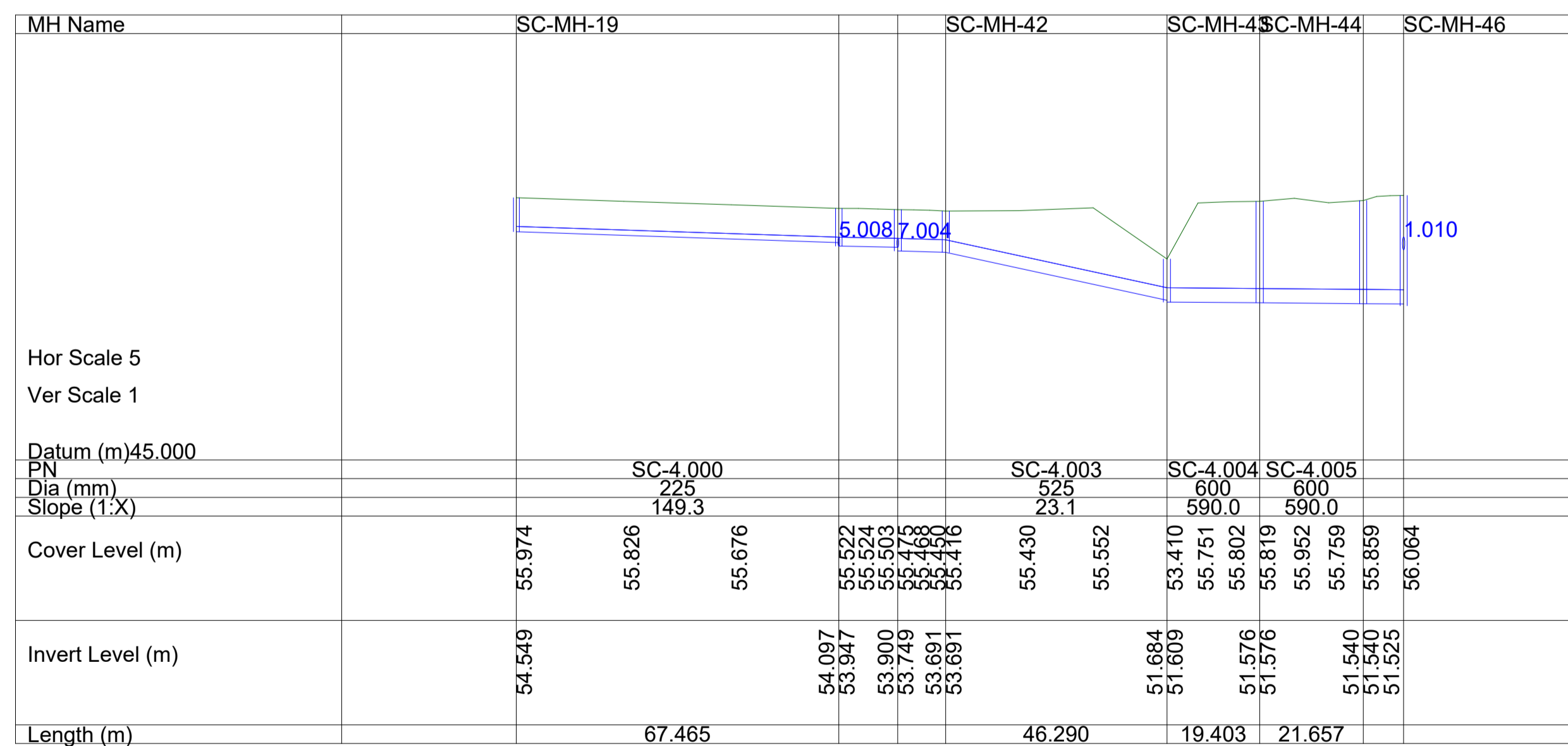
SURFACE WATER NETWORK: SC-4.000 - SC-4.006
