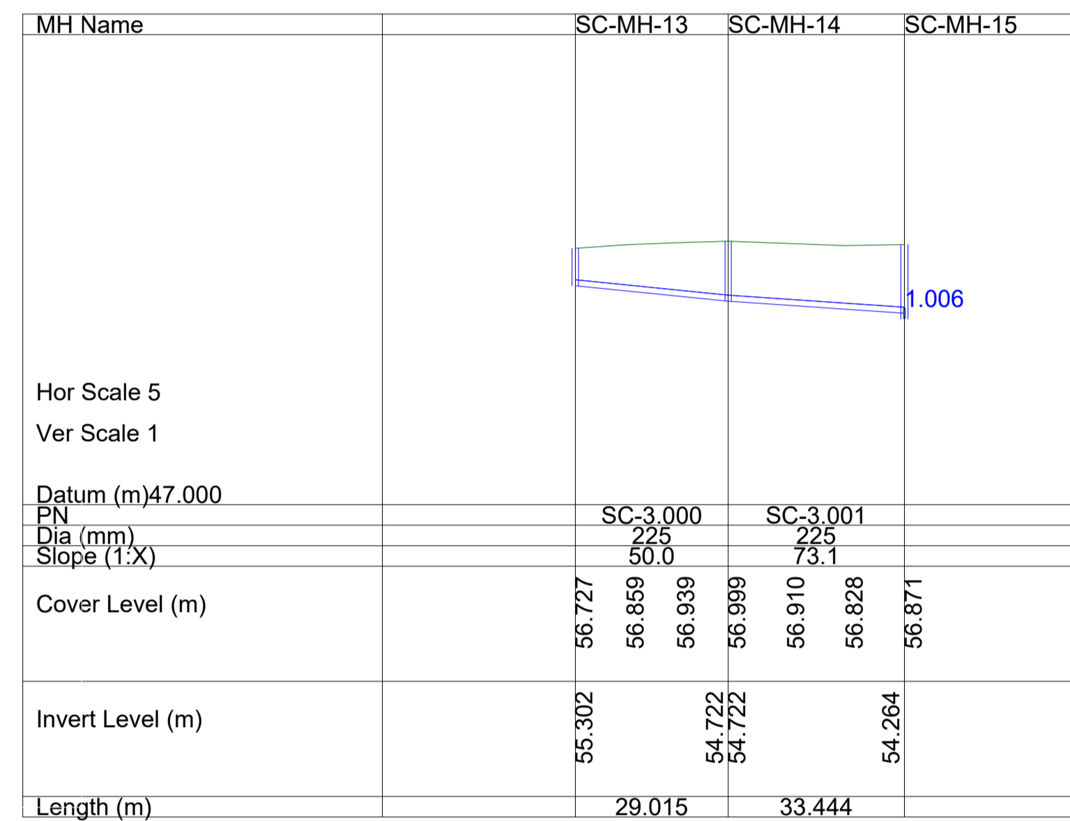
SURFACE WATER NETWORK: SC-3.000 - SC-3.001
