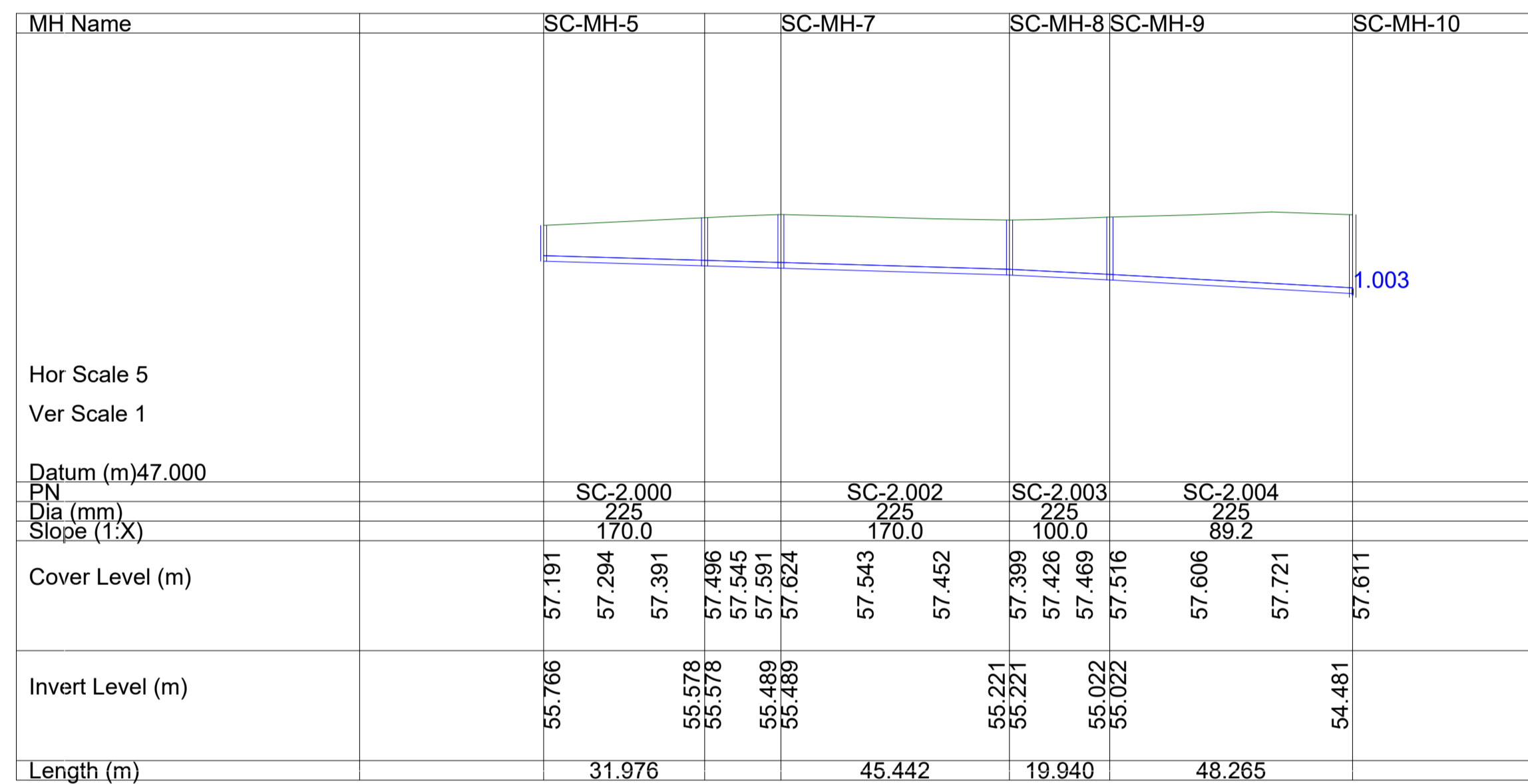
SURFACE WATER NETWORK: SC-2.000 - SC-2.004
