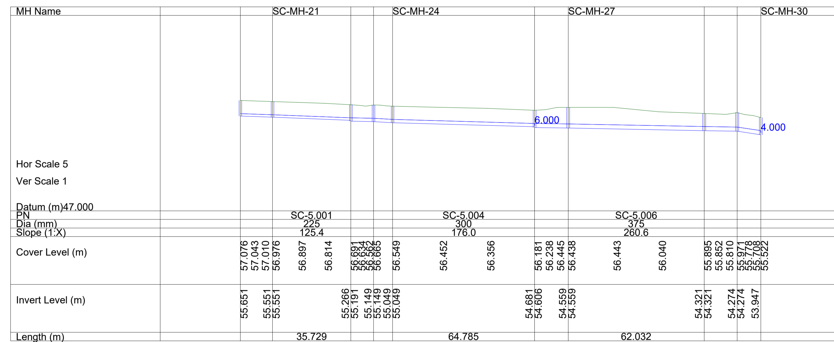
SURFACE WATER NETWORK: SC-5.000 - SC-5.008
